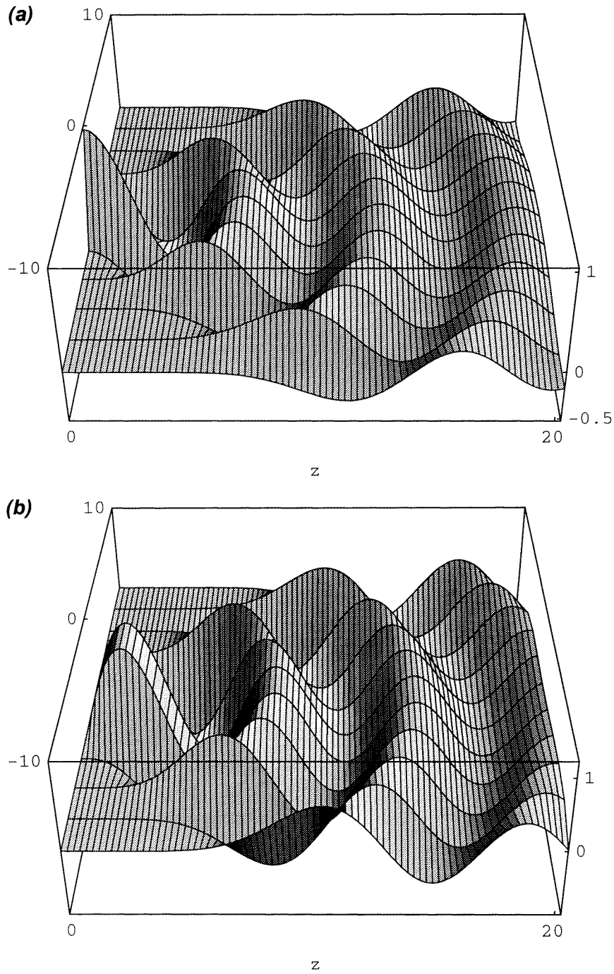
Figure 3. Discrete waveforms in the q - z plane obtained from the initial condition \psi^{(0)} (a single 1 at m = 0 ) under z -evolution generated by the discrete optical Hamiltonian (4.6). (a) Interpolating linearly between even- m points; and (b) between odd- m points. The former are interpreted as field values and the latter as the z -normal derivatives.
