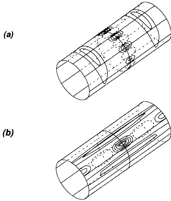
Figure 7. Marginal distribution on the cylinder of the Wigner of Schrödinger cat states composed of two Gaussian vectors (4.7). (a) Two parallel narrow Gaussian beams separated in position. (b) Two overlapping wide Gaussian beams at different angles.
