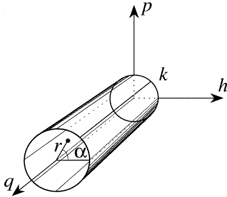
Figure 4. The Wigner function W(\psi|q, p, h) on three-dimensional space (q, p, h) is different from zero inside a cylinder whose axis is (q, 0, 0) and whose squared radius is p^2 + h^2 = k^2 , determined by the unirrep label k = \lambda^{-1} \in \mathbb{R}^+ . On the surface of the cylinder there is an inverse-square-root singularity.
